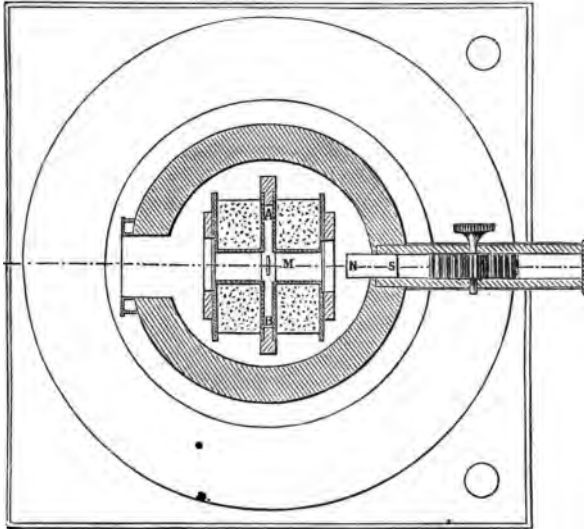
Sectional Plan.
